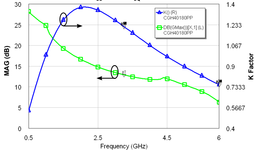
Simulated Maximum Available Gain and K Factor of the CGH40180PP
